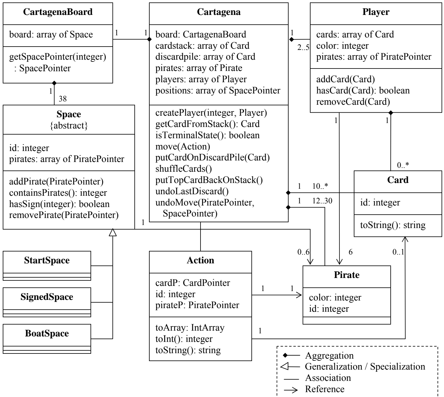
Figure 6.1: A UML class diagram of the Cartagena classes. For UML details see for instance [Eriksson and Penker, 1999].
