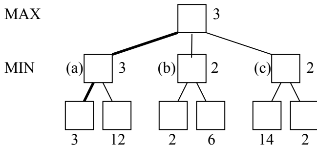
Figure 3.2: Minimax with evaluation values
