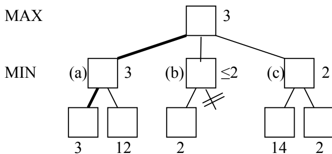
Figure 3.3: Minimax with evaluation functions and Alpha-Beta pruning
