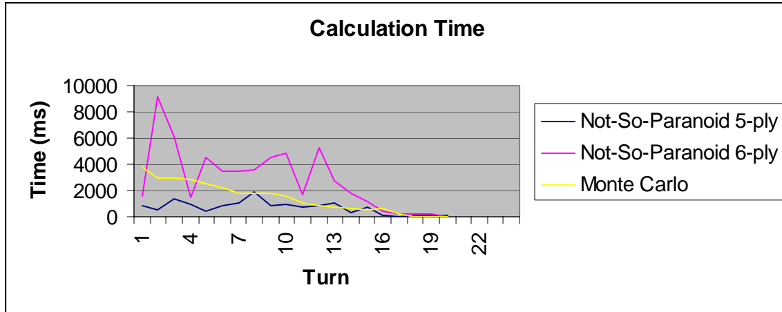
Figure 7.3: Monte Carlo calculation time in a 3-player game together with a 5-ply and 6-ply Not-So-Paranoid player with extended pruning
