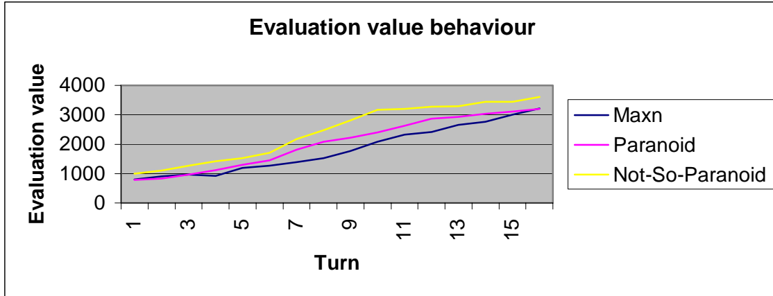
Figure 7.2: The evaluation value in a game between Max^n , Paranoid and Not-So-Paranoid p (using 3-ply search)
