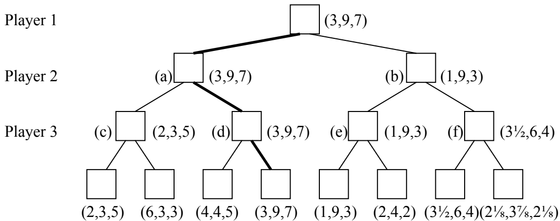
Figure 3.4: Max^n search tree example
