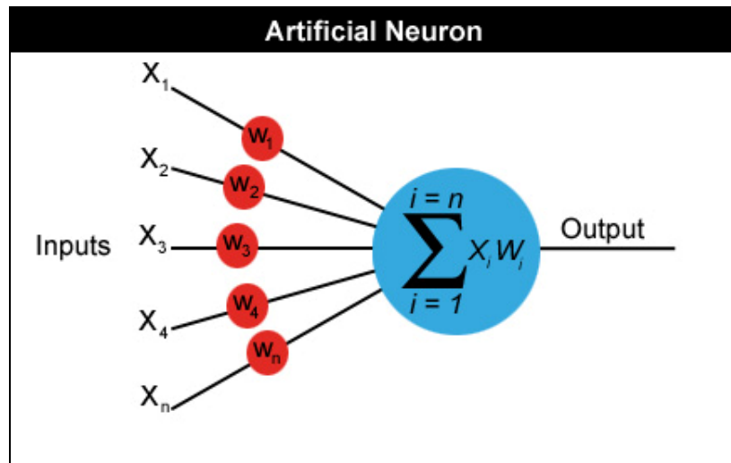
Figure 4.2: A unit (an artificial neuron).
