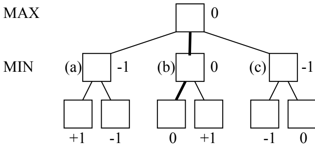
Figure 3.1: a 2-ply Minimax search tree with win, loss and draw utilities in the nodes
