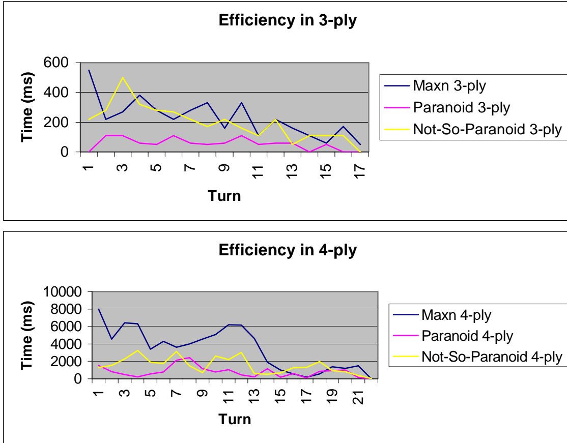
Figure 7.1: Calculation times in a 3-ply and 4-ply search for Max^n , Paranoid and Not-So-Paranoid p in a typical game
