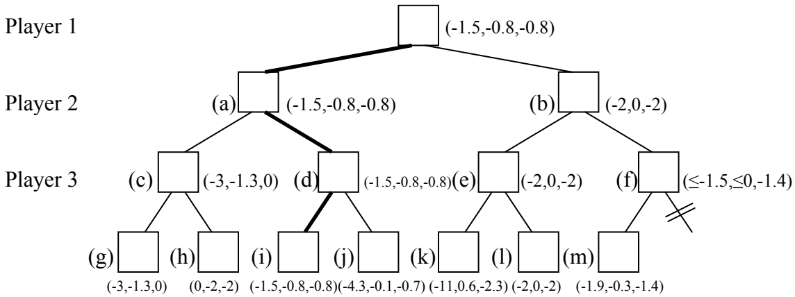
Figure 5.2: Not-So-Paranoid search tree example with pruning
