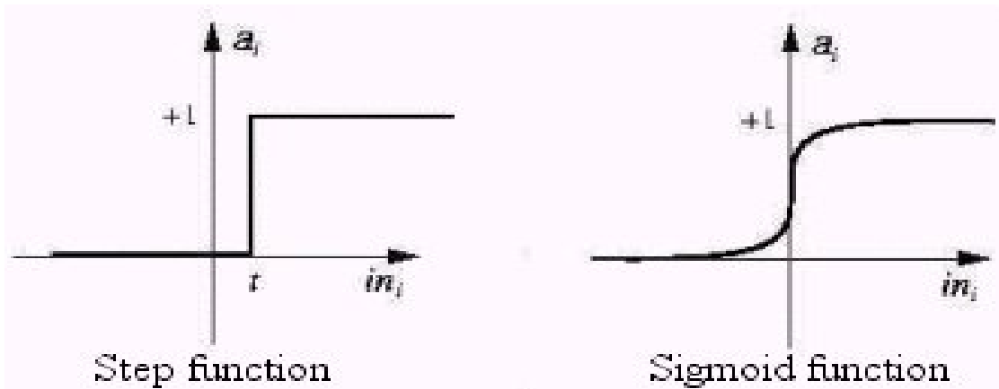
Figure 4.3: Two activation functions: on the left side the step function and on the right side the sigmoid function.
