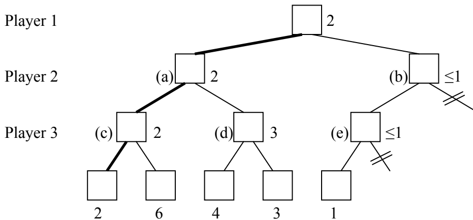
Figure 3.5: Paranoid search tree example
