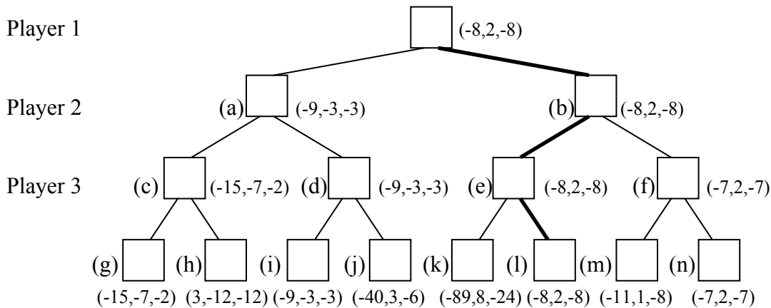
Figure 5.1: Not-So-Paranoid search tree example
